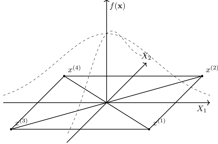
Figure 7: A 2D standardised Gaussian and its network realisation
